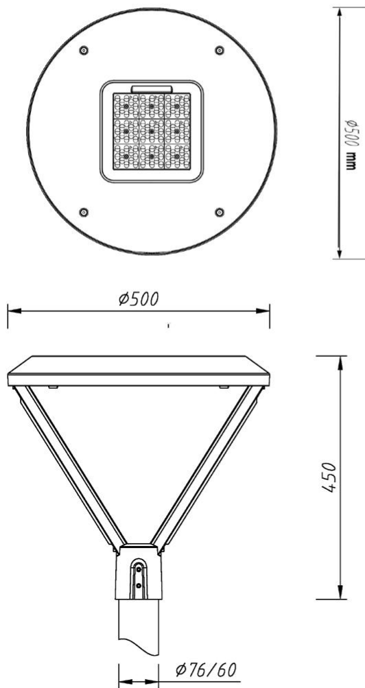
GSL08 D:Post top mounted
