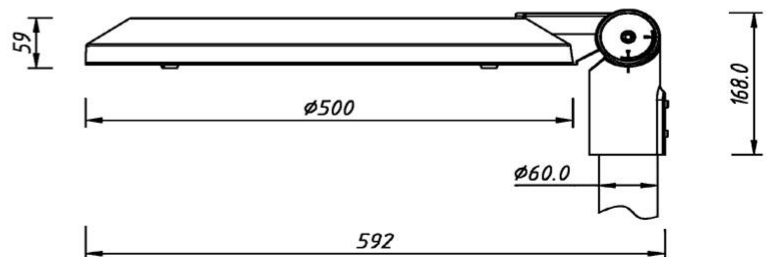
GSL08 S :Side entry mounted
