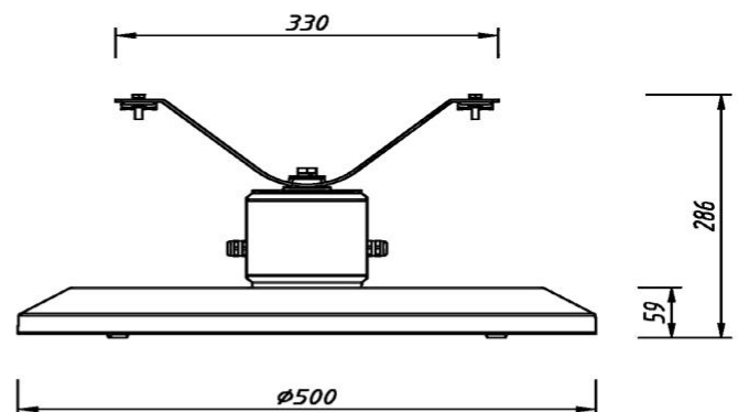
GSL08 L :Suspended mounted
